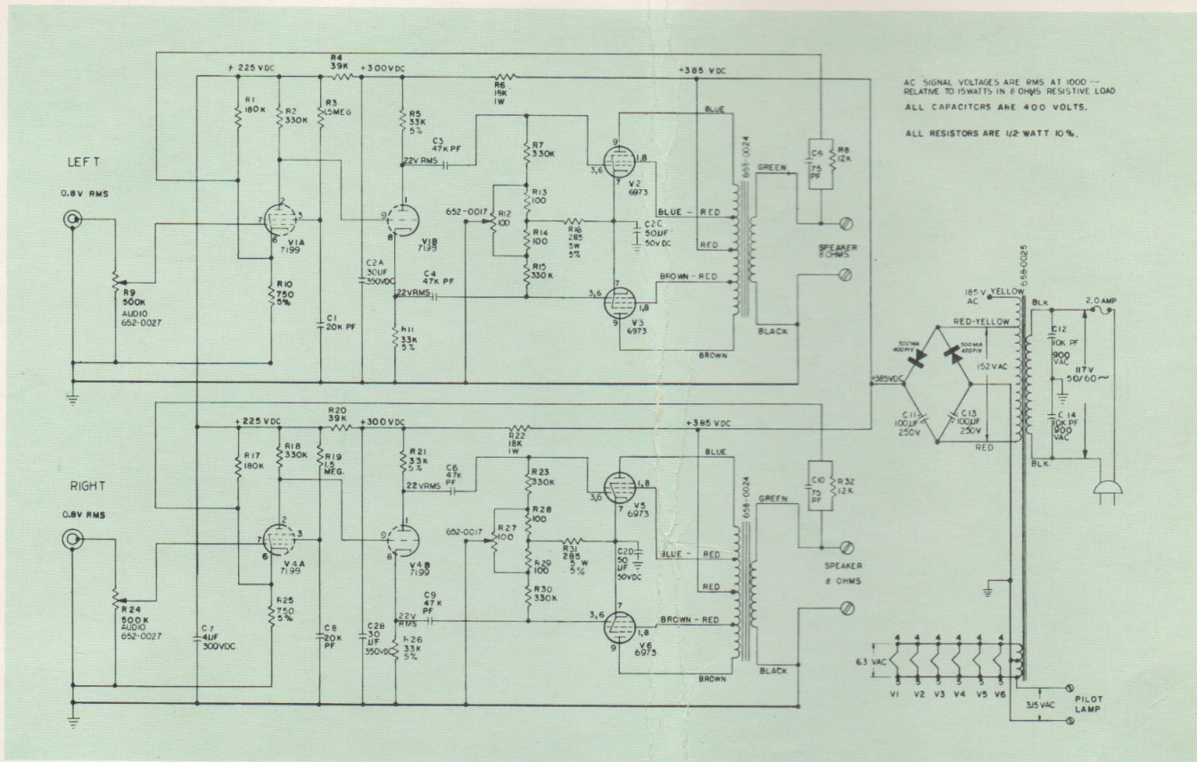
STEREO AMPLIFIER
